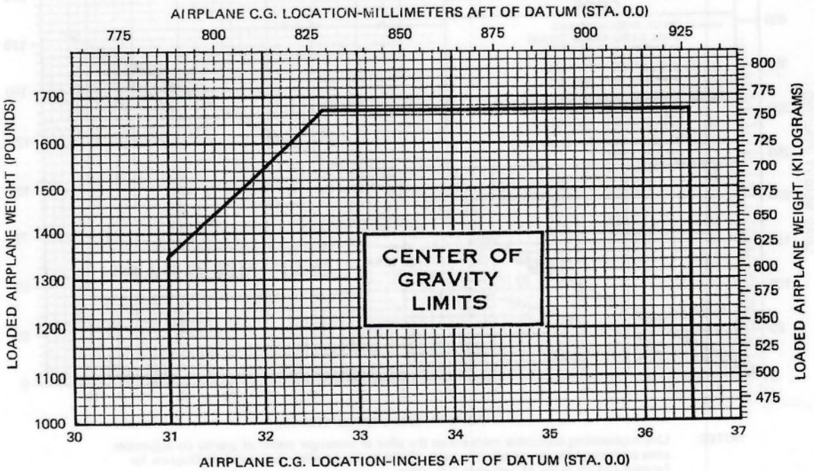
Figure 6-9. Center of Gravity Limits
